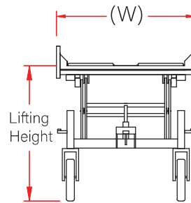
Front View Model : BTT-1 (Adjustable Height)
